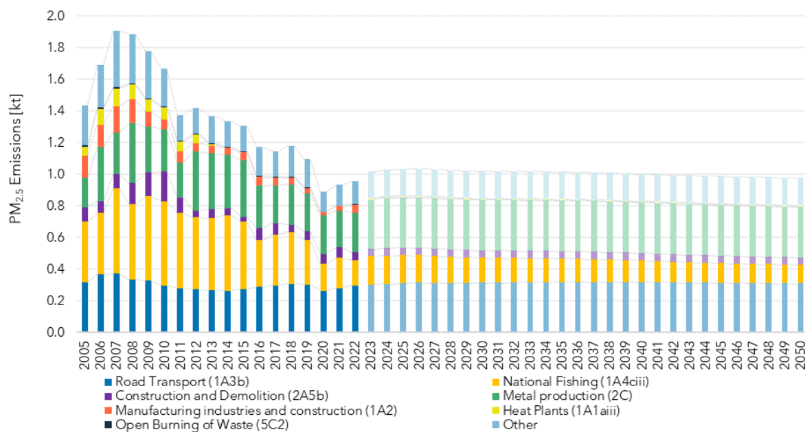
Figure 9.5 PM 2.5 emissions by main sources. Historical data and projections, 2005-2050.
