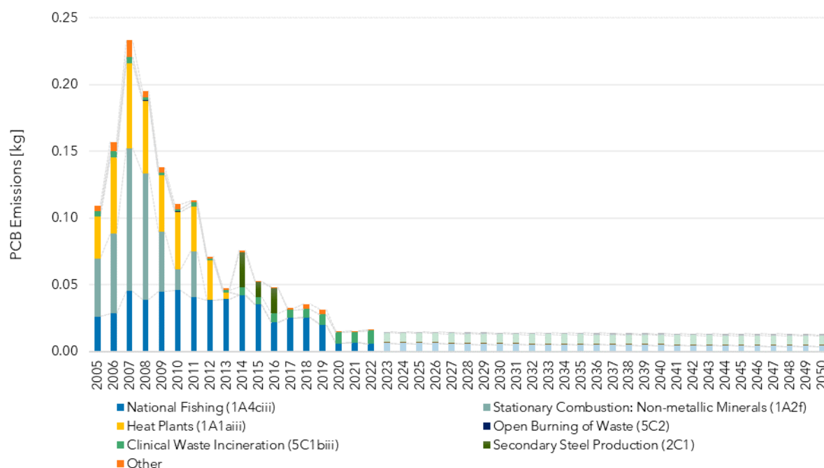
Figure 9.13 PCB emissions by main sources. Historical data and projections, 2005-2050.
