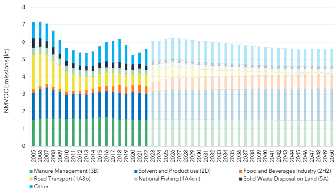
Figure 9.2 NMVOC emissions by main sources. Historical data and projections, 2005-2050.
